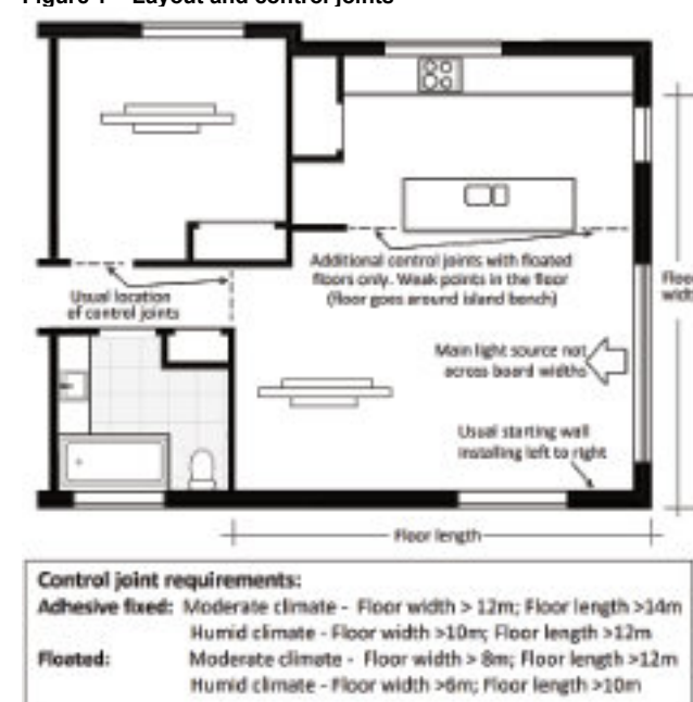
Figure 2 – Installation
