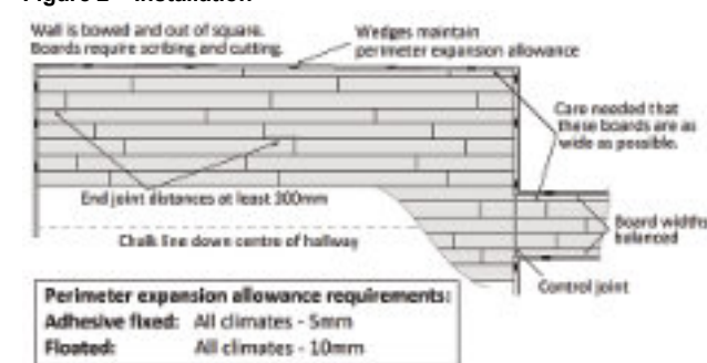
Figure 3 – Scribing
